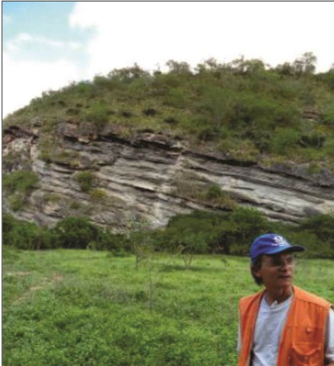
Sergipana Foldbelt, northeastern Brazil, 2013.
